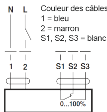
Câblage LF230S
