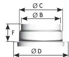
Manchette (Incluse)
