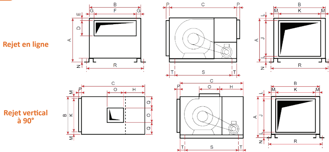
Dimensions (mm)
