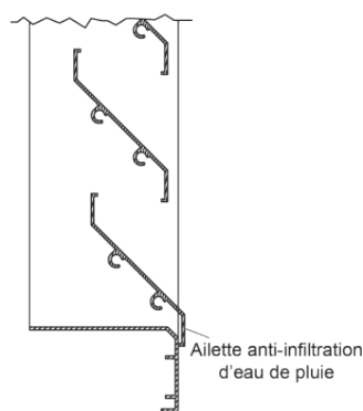
Ailette anti-gouttes
